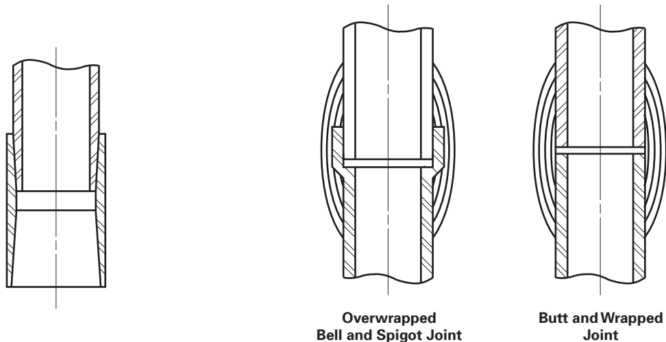
FIG. A328.5.6 FULLY TAPERED HERMOSETTING ADHESIVE JOINT
