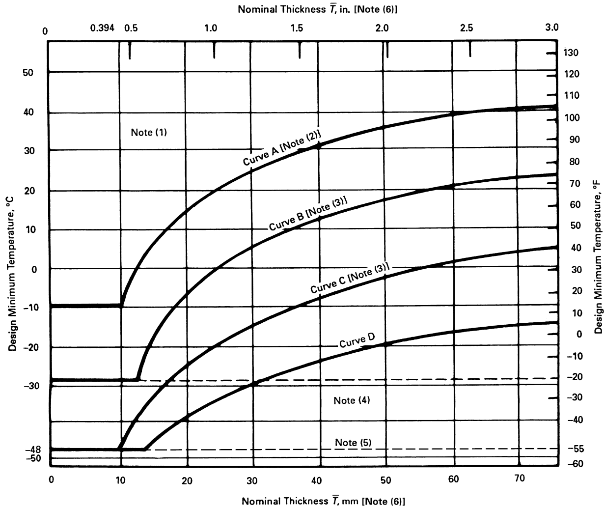
(16) Fig. 323.2.2A Minimum Temperatures Without Impact Testing for Carbon Steel Materials (See Table A-1 or Table A-1M for Designated Curve for a Listed Material; see Table 323.2.2A for Tabular Values)
